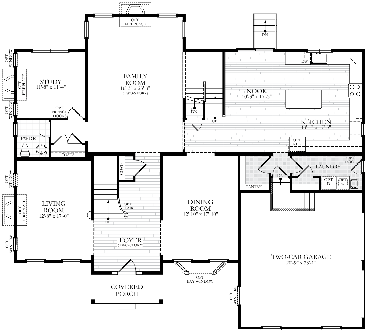
FIRST FLOOR
